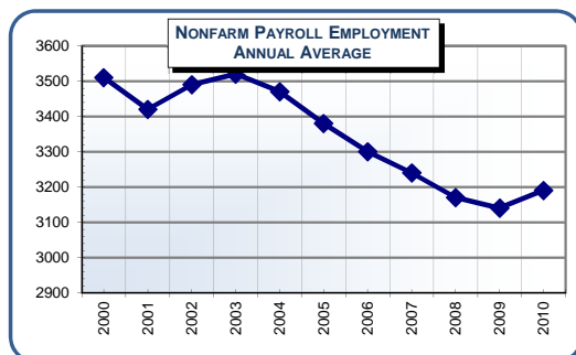
Benchmark 2010
